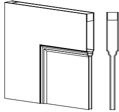
STEPPED STICKING
